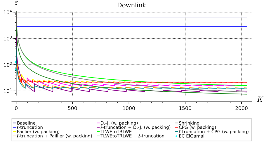
Fig. 1: Comparison of expansion factors for the downlink ciphertext compression methods studied in this paper and \ell found using Prop. 1 ( t = 16 )
