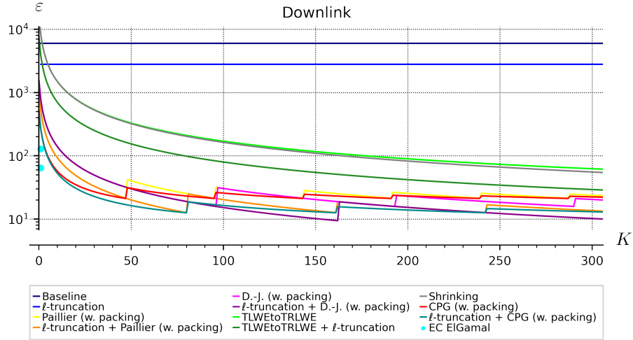
Fig. 2: Comparison of expansion factors for the downlink ciphertext compression methods studied in this paper for K \leq 300 and \ell found using Prop. 1 ( t = 16 )
